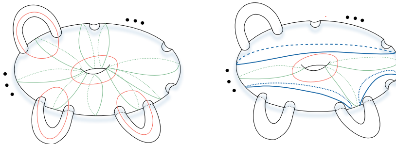
FIGURE 1. A diagram of the Gervais curves on S_{g,b} . On the left are \alpha_1, \dots, \alpha_{2g+b-2} (appearing as meridians of the central torus) and \beta_1, \dots, \beta_g (with \beta_1 as the longitude of the central torus). For every pair \alpha_i, \alpha_j , there is a corresponding curve \gamma_{ij} ; the figure on the right shows three of the \gamma_{ij} . The star relations are formed by twists around seven curves in the configuration depicted on the right; the central curve \beta_1 is always used. Note that each such relation is supported on a three-times punctured torus.
